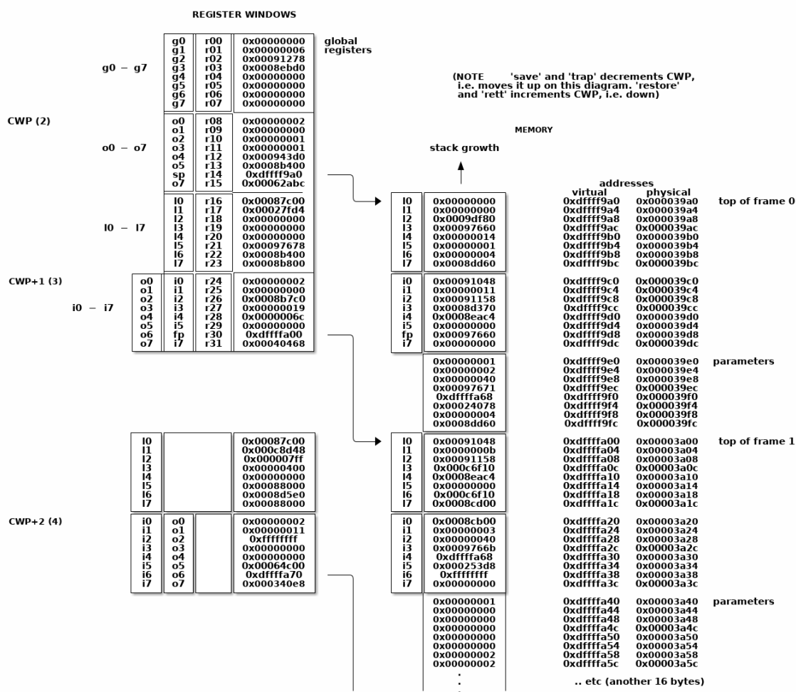
Fig. 18.3: Figure 4 - Sample stack contents
