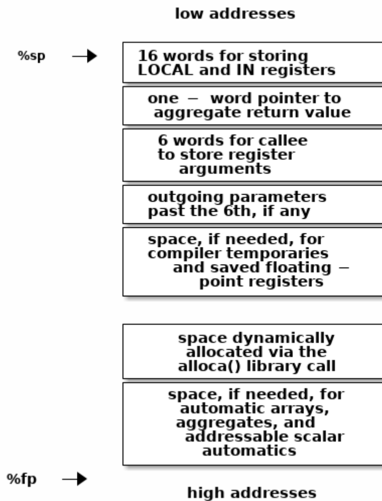
Fig. 18.2: Figure 3 - Stack frame contents
