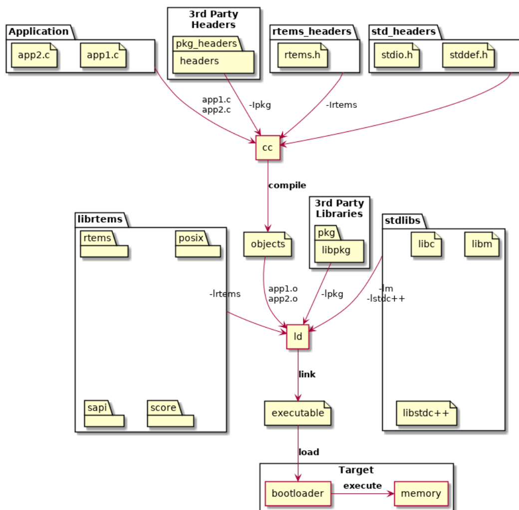
Fig. 8.2: Building an Application
