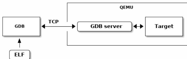
Fig. 8.4: QEMU Executable Debugging
