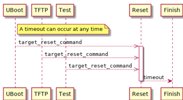
Fig. 9: Target Timeout
