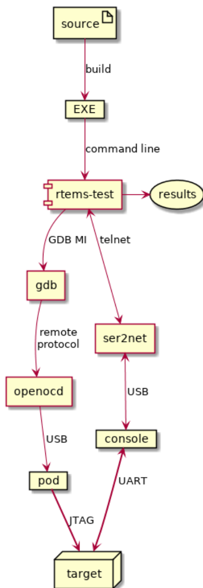
Fig. 4: RTEMS Tester using GDB and JTAG
