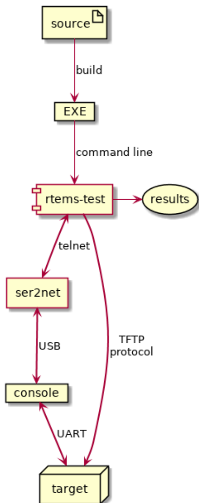
Fig. 10.5: RTEMS Tester using TFTP and U-Boot.
