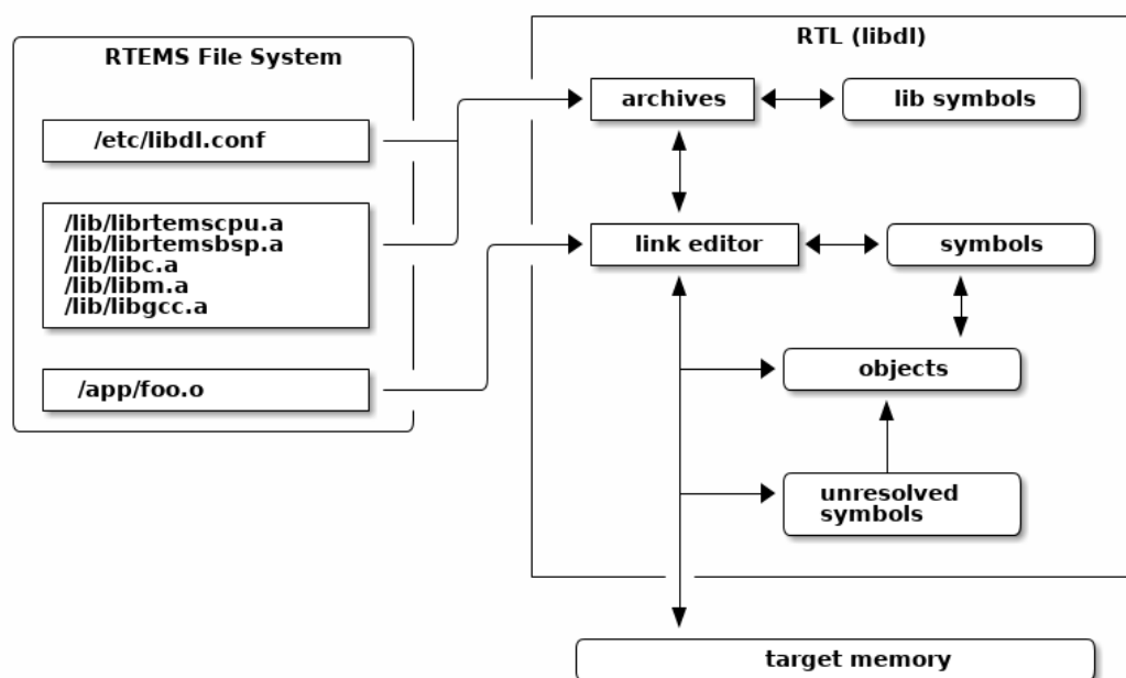
Fig. 9.7: Run Time Loader (libdl)
