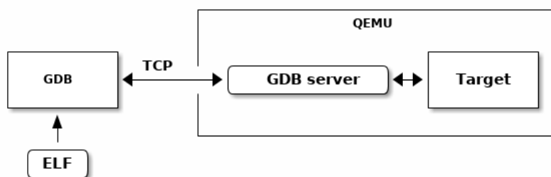
Fig. 9.4: QEMU Executable Debugging
