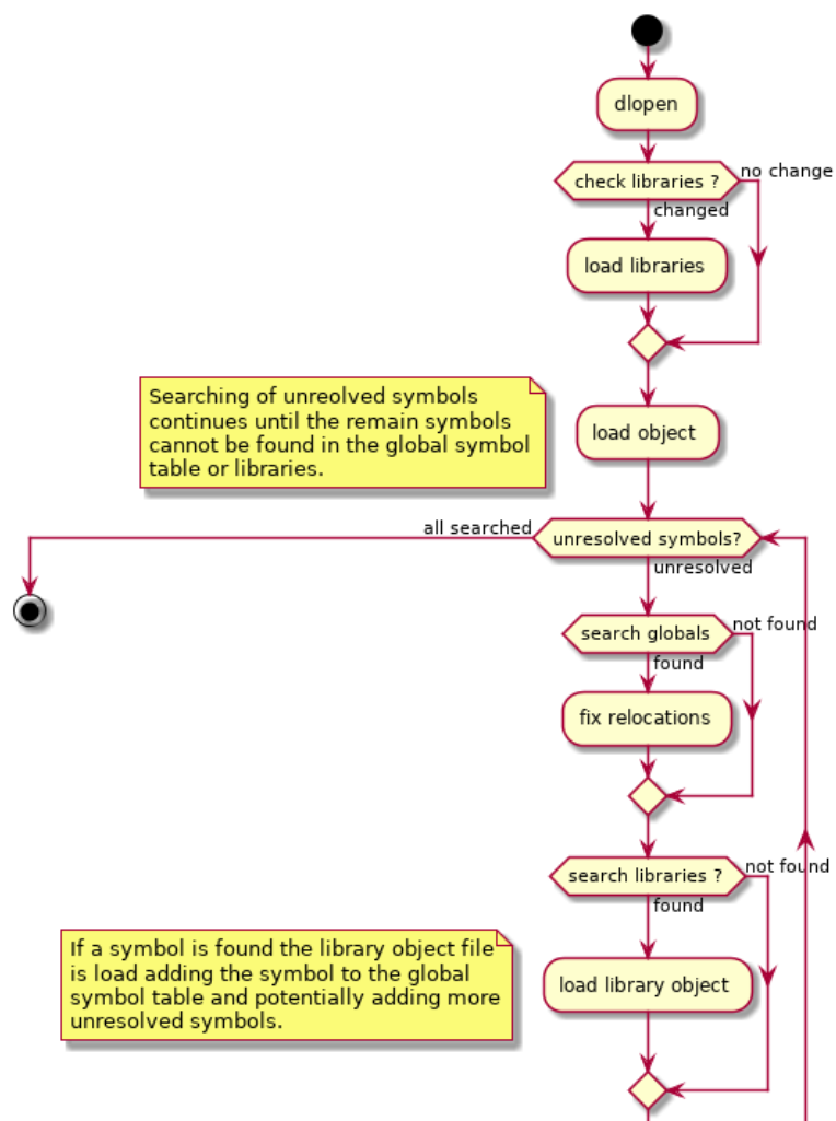
Fig. 9.8: Loading Executable Object Files
