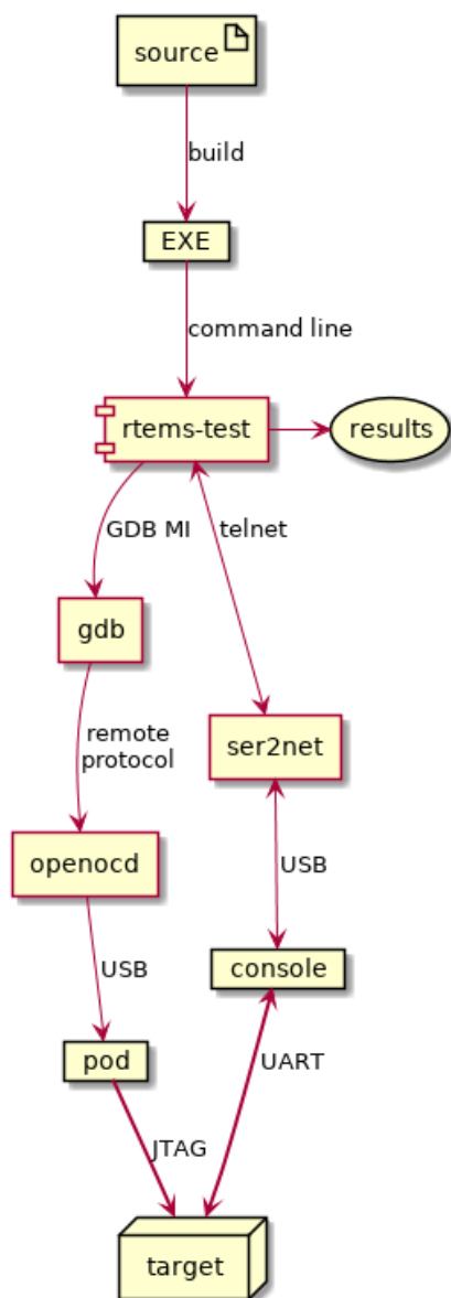
Fig. 10.4: RTEMS Tester using GDB and JTAG
