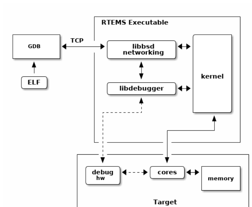
Fig. 9.6: Libdebugger Executable Debugging
