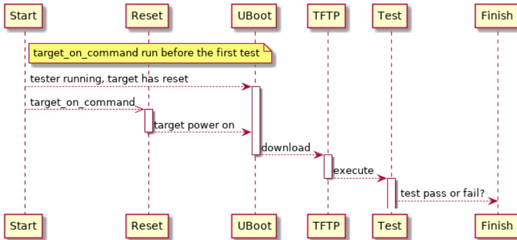
Fig. 10.6: Test Pass and Fail Sequences
