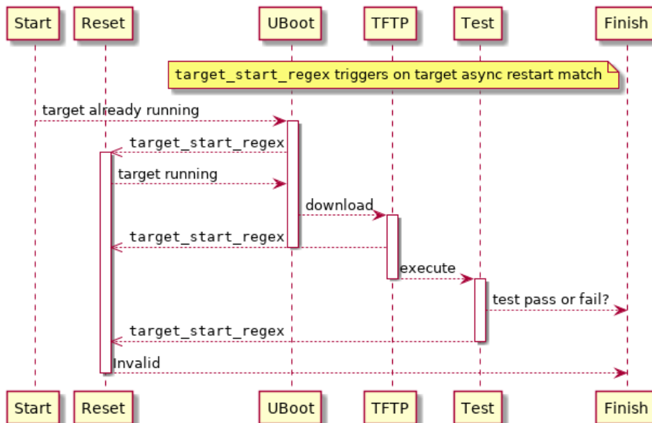
Fig. 10.7: Target Start Filter Trigger
