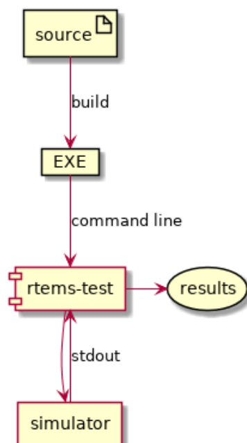
Fig. 10.3: RTEMS Tester Simulation
